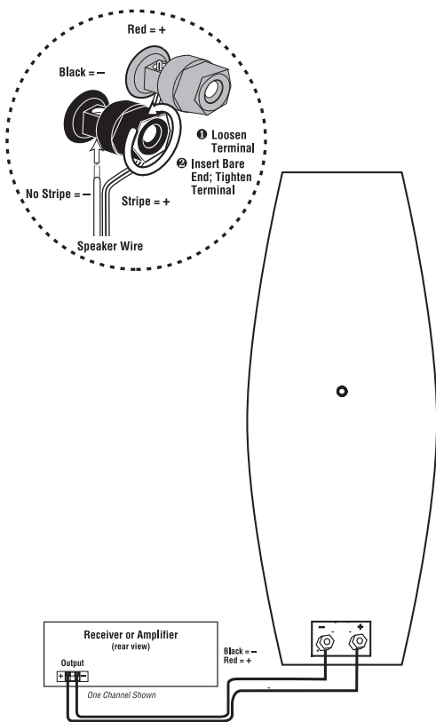
Figure 3. Wiring diagram shows polarity connections for one channel of a home theater system.
